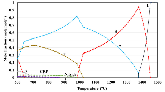
Fig. 9 – Equilibrium phase diagram of CuHIP sample.
